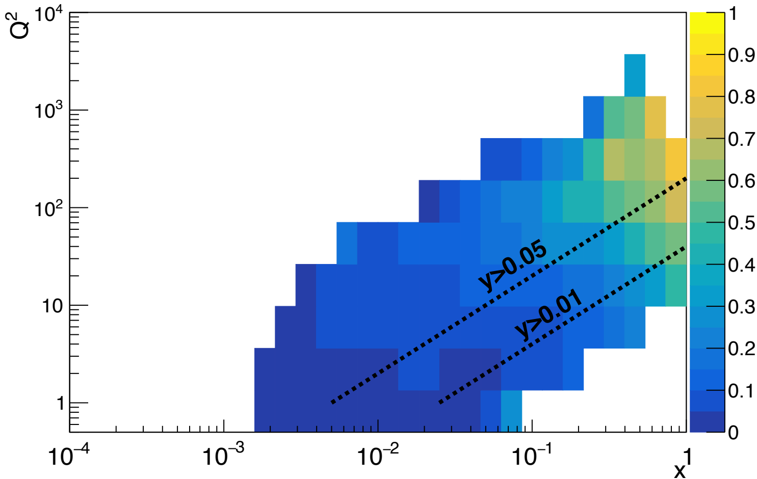
Fraction of events staying in bin (10x100)
