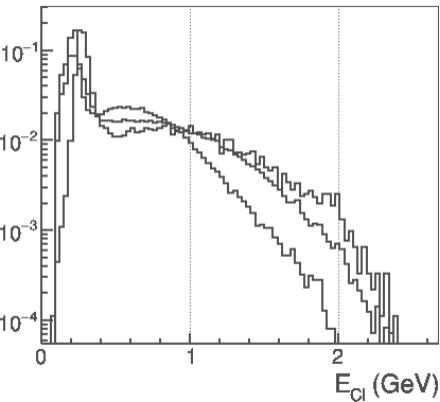
EMCal response to 2 GeV/c \pi^-
