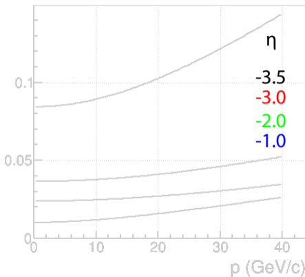
\Delta p/p vs p (GeV/c)
