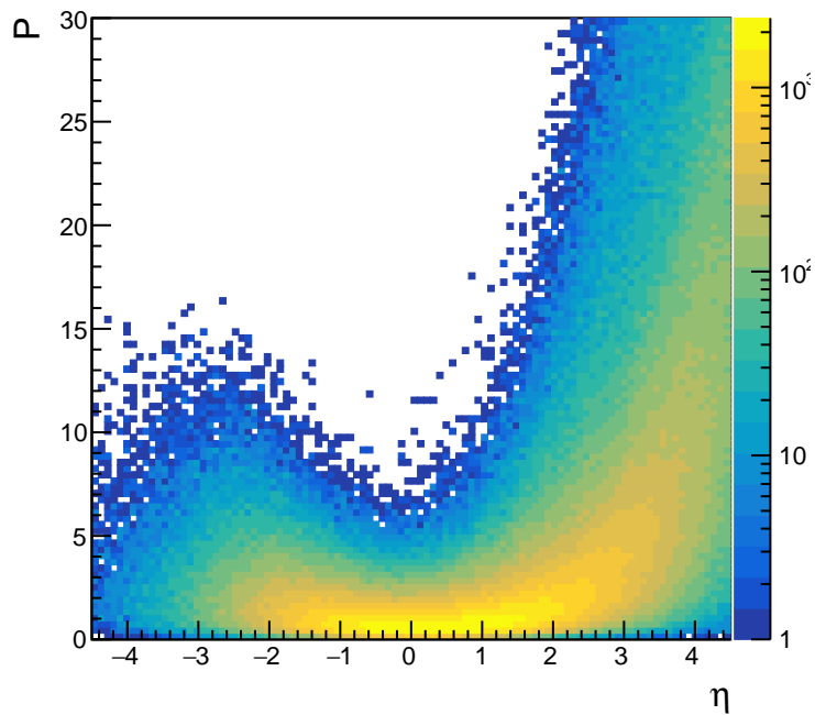
gpion_eta_mom
