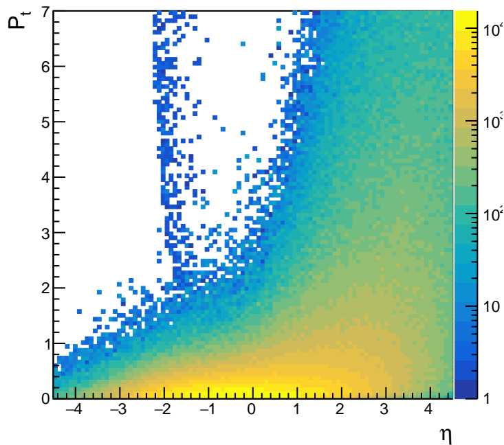
rpion_eta_pt
